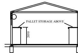
SECTION B
