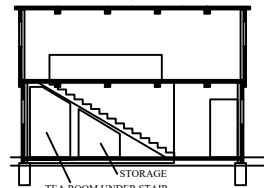
SECTION D
