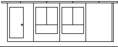
FRONT ELEVATION COURTYARD SIDE
