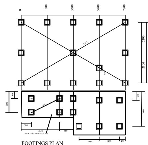
FOOTINGS PLAN
