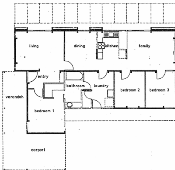
UNIBUILD “PASSIVE” SOLAR HEATING DESIGN DETAIL
