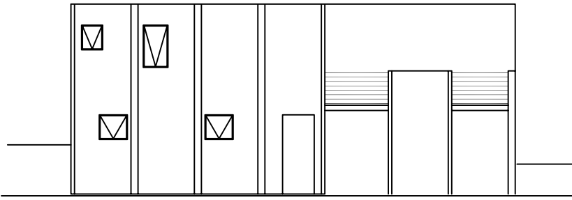
EAST ELEVATION
