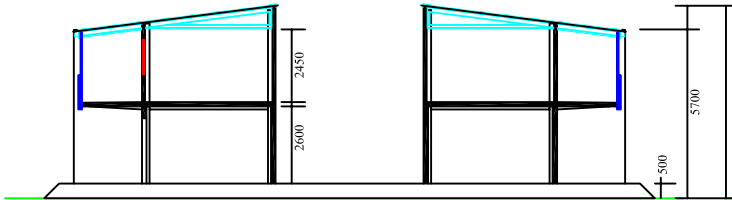
SECTION A
