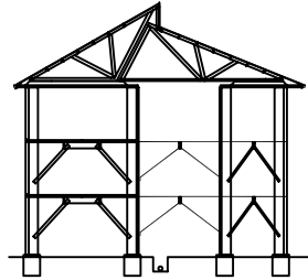
ERECT ROOF TRUSS UNITS, INSULATION & SHEETING. TEMP FORMWORK UNITS, PRECAST FLOOR SLABS & CONDECK PLUMBING & ELECTRICAL "ROUGH IN", REINFORCING TO 1ST & 2ND FLOOR SLABS.
