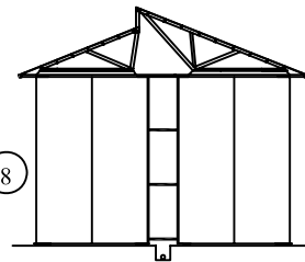
FIX PRECAST END WALLS FIX END PRECAST ROOF PANELS
