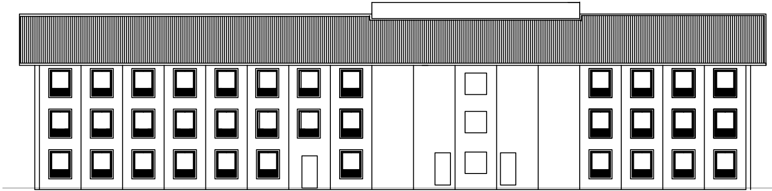
REAR ELEVATION
