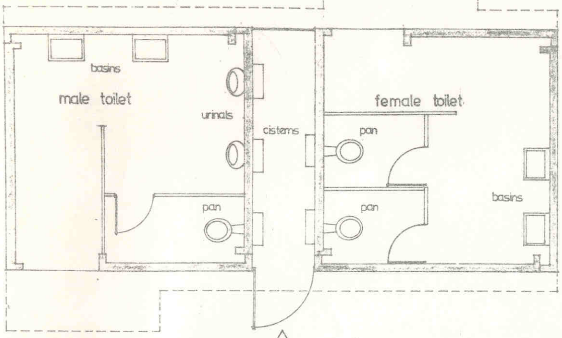
plan
