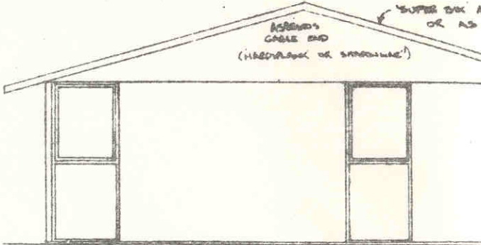
SIDE ELEVATIONS
