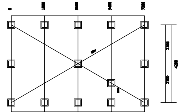
FOOTINGS PLAN
