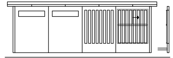
REAR ELEVATION
