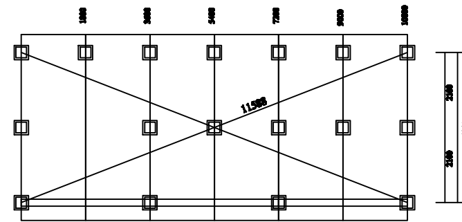
FOOTINGS PLAN
