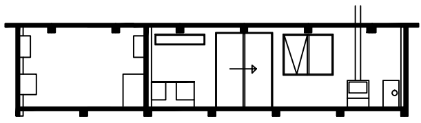
SECTION B
