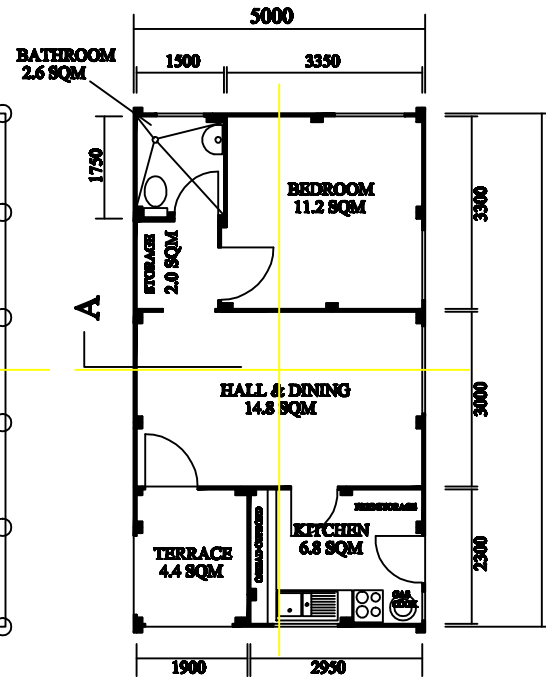
FLOOR PLAN
