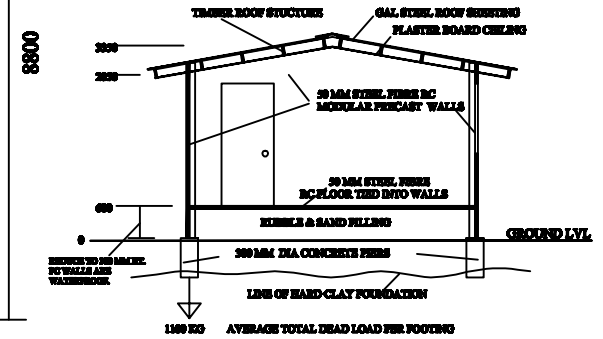
SECTION A
