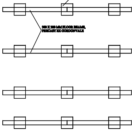
FOOTING PLAN
