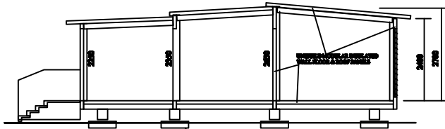
SECTION A
