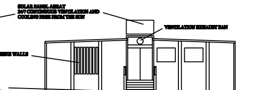
SOUTH (REAR) ELEVATION
