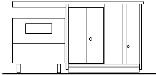
EAST (FRONT) ELEVATION
