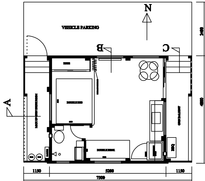
FLOOR PLAN
