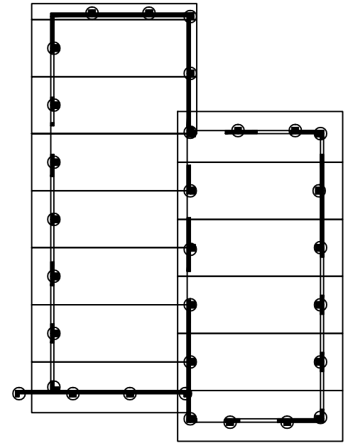
STRUCTURAL SHELL FOOTING PADS, PRECAST WALLS, PRECAST ROOF
