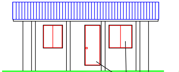
FRONT ELEVATION DOOR & WINDOW OPENINGS
