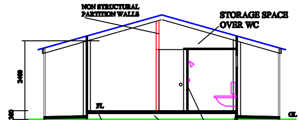
SECTION A
