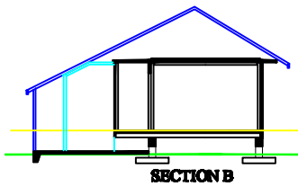
SECTION B
