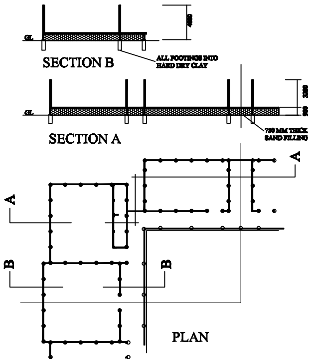
GROUND FLOOR SLAB ON FILL
