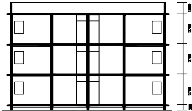
SECTION A
