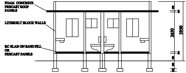
SECTION A
