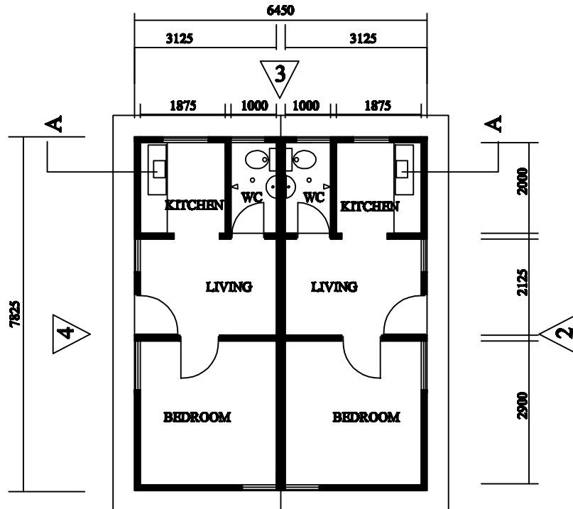
1 PLAN (NO 2 UNITS)
