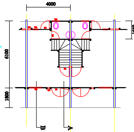
PLAN - LOWER
