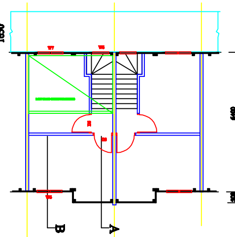
PLAN - UPPER
