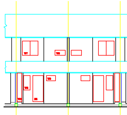
REAR ELEVATION
