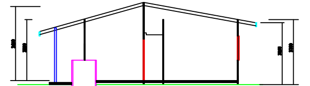
SECTION B
