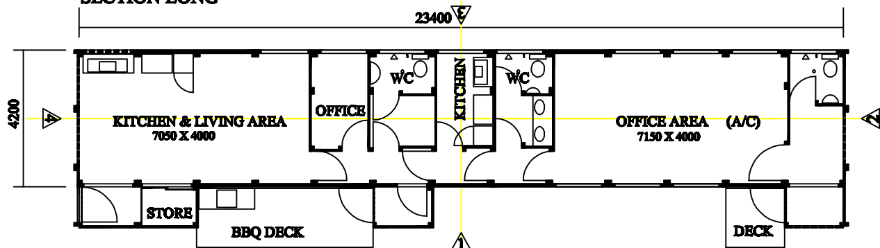
SECTION LONG
