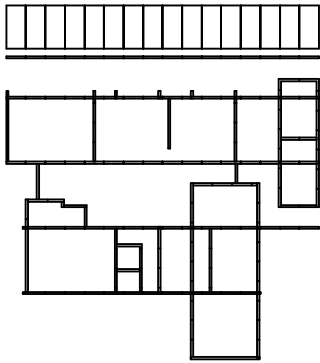
AREA - 1015 SQM (NO 141 X 4M X 1.8M) PRECAST WALLS (FL 1)
