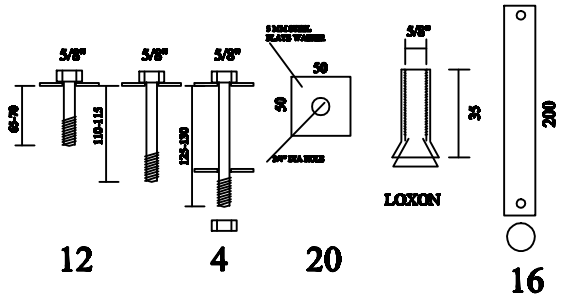
PRECAST FIXINGS
