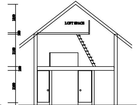
SECTION B (LOFT OPTIONAL)
