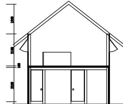
SECTION A
