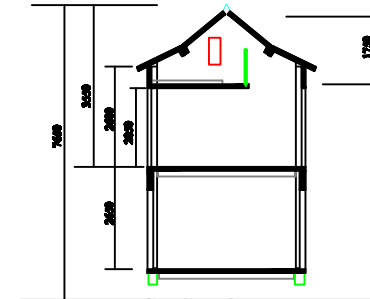
SECTION B
