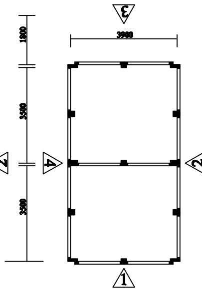
PLAN TOP FLOOR
