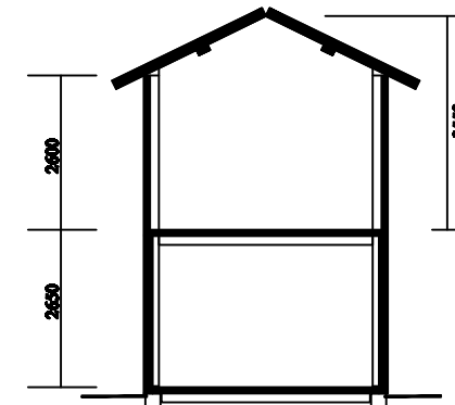
SECTION A
