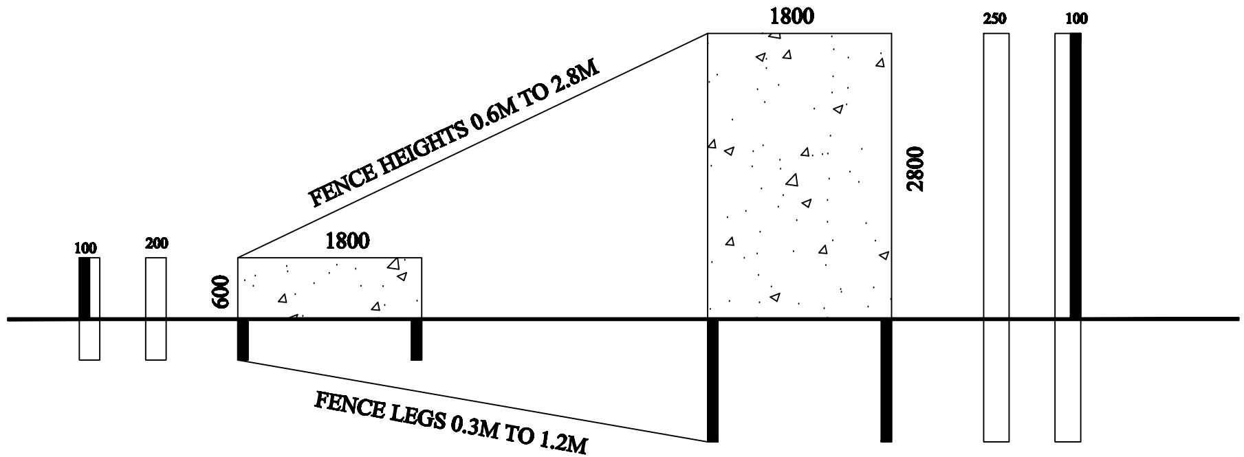
FENCE WALL PANEL RANGE
