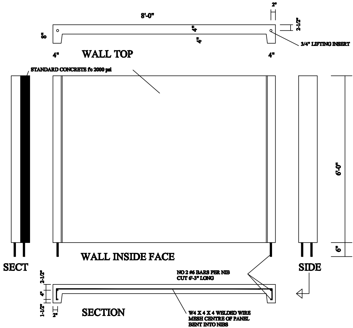
TYPICAL FENCE WALL
