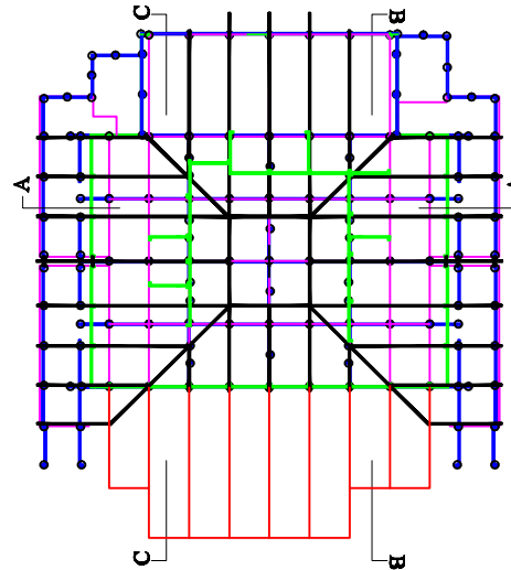
PLAN (COMPOSITE)
