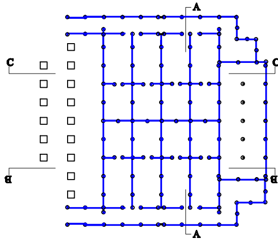
FOOTINGS, BASEMENT WALLS
