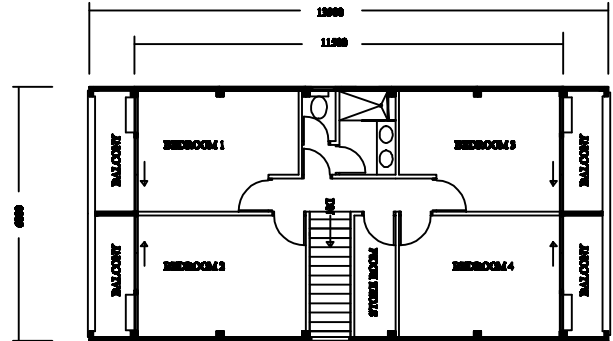
UPPER FLOOR
