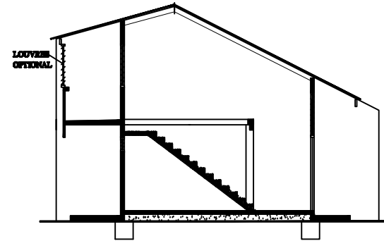
SECTION A
