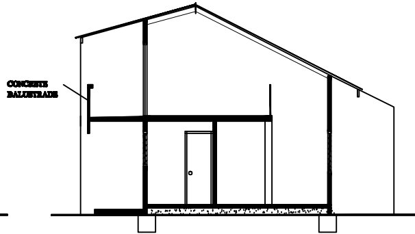
SECTION B
