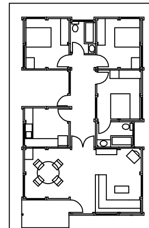
FLOOR PLAN 6004
