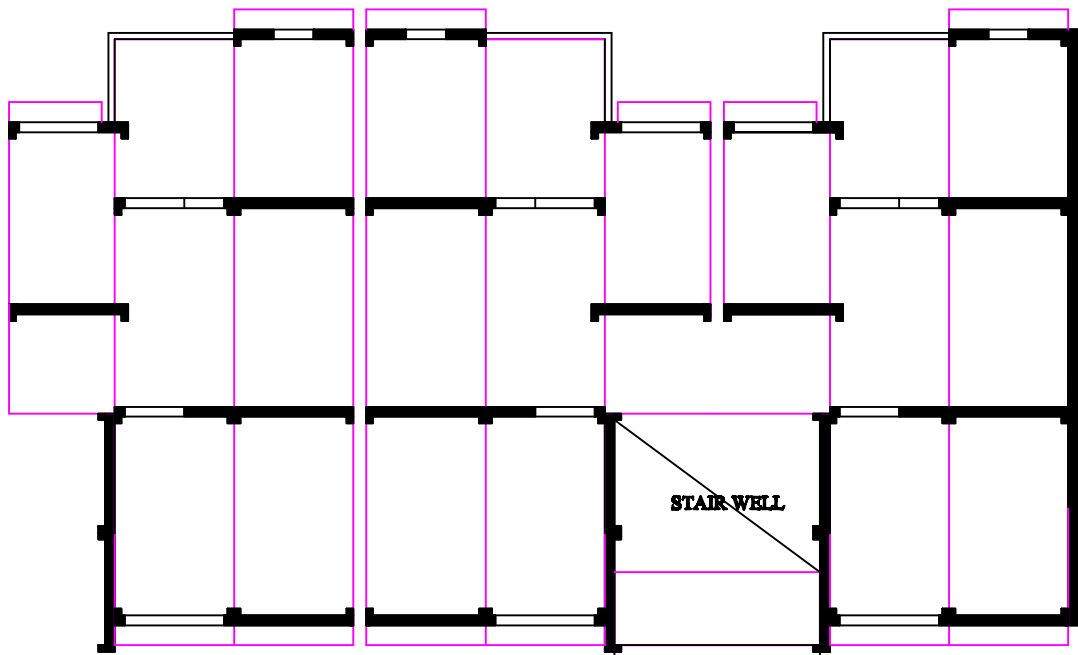
PRECAST WALL & FLOOR COMPONENTS
