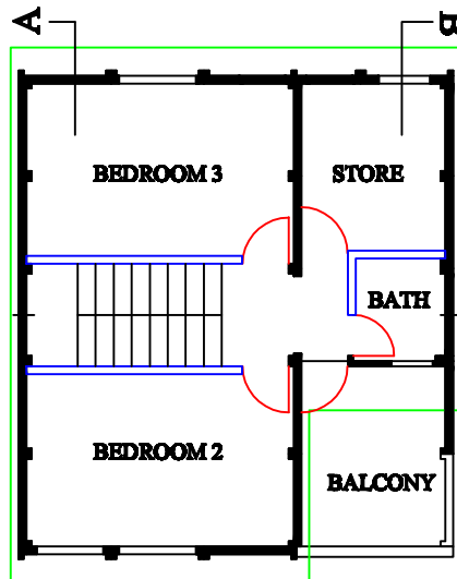
UPPER FLOOR
