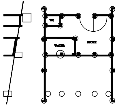
FOUNDATIONS
