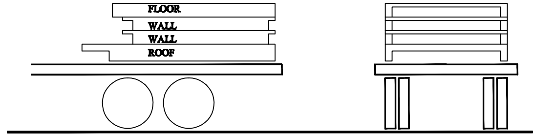
TRUCK PANEL LOADING PER BAY
