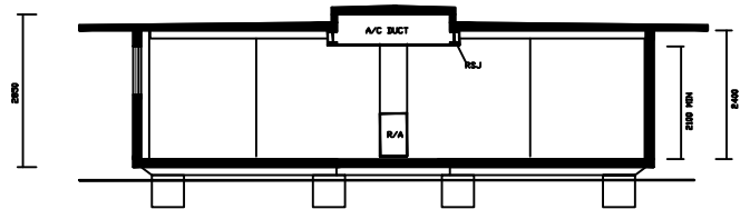
SECTION E-E
