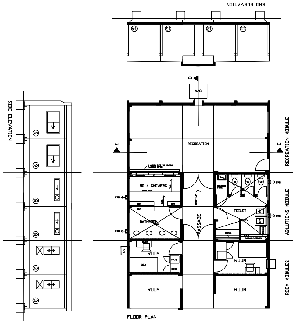
FLOOR PLAN
