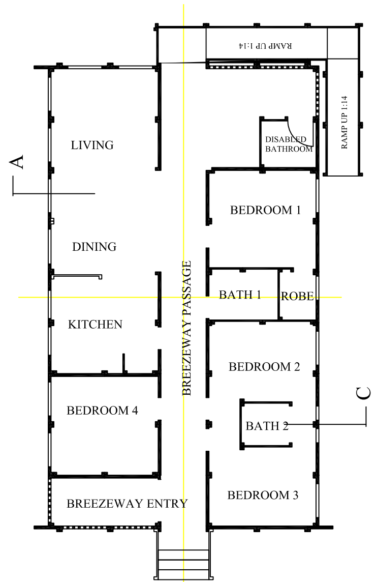
STRUCTURAL UNIBUILD SHELL DISABLED PERSONS VARIATION
