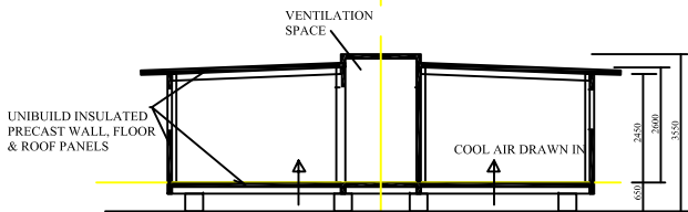
SECTION A
