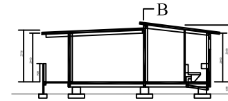
SECTION D
