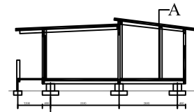
SECTION E
