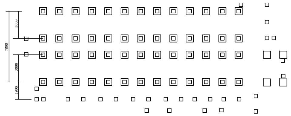
FOOTINGS PLAN
