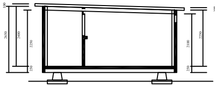
SECTION C
