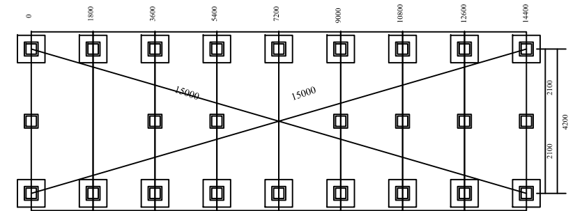
FOOTINGS PLAN
