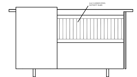
WEST ELEVATION
