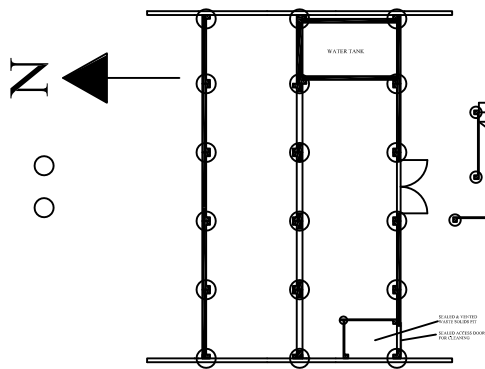
FOOTINGS & FOUNDATION WALLS
