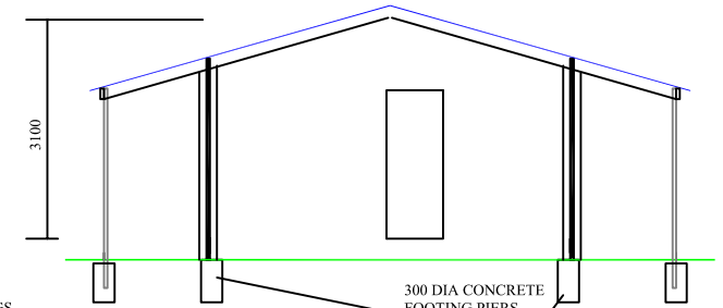
SECTION A
